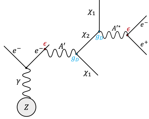
Fig. 2.1 Production of A' via a dark bremsstrahlung reaction e^- Z \rightarrow e^- Z A' and subsequent semi-visible decay A' \rightarrow \chi_2 \chi_1; \chi_2 \rightarrow \chi_1 A'^* \rightarrow \chi_1 e^+ e^- .
